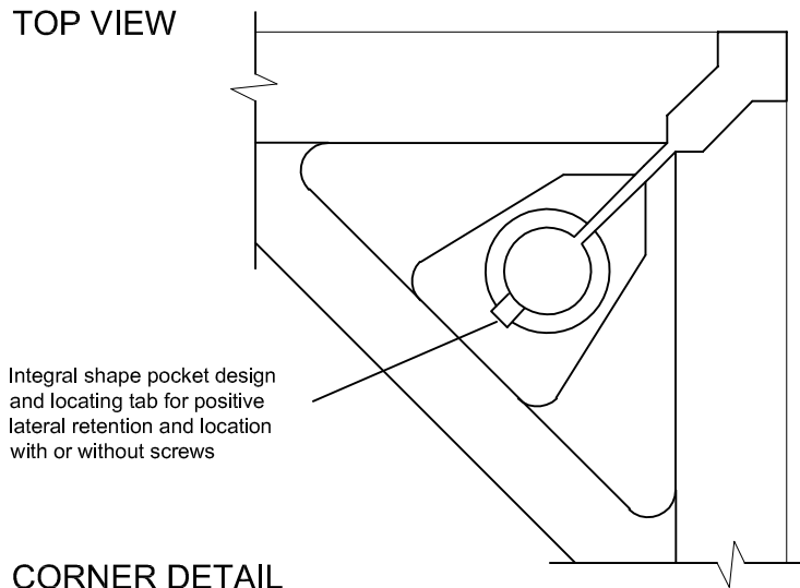
CORNER DETAIL
